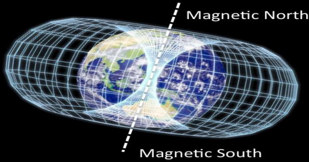
BEFORE Pole Reversal
