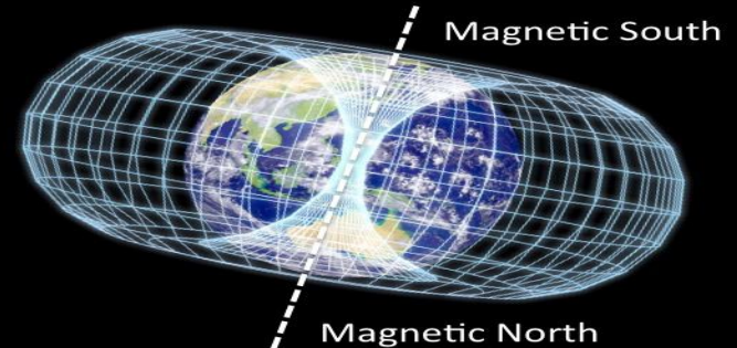
AFTER Pole Reversal
